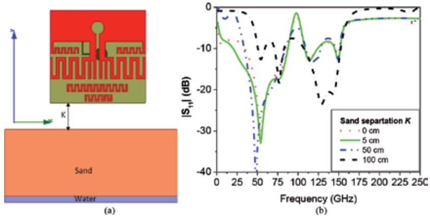
Figure 20. (a) The GPR antenna system for water detection and (b) the effect of K on proposed antenna reflection coefficient [37].
