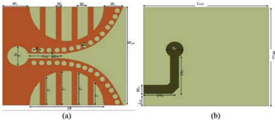
Figure 3. Geometry of the proposed Vivaldi antenna (a) ground plane and (b) feed line.
