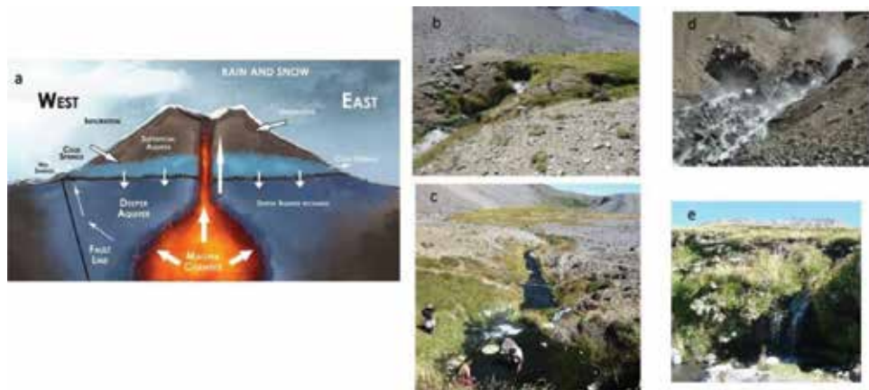
Figure 5. (a) Scheme of the plausible groundwater system at one volcanic complex; (b) headwaters of the Diguillín River at a thermal spring; (c) Diguillín River; (d) hot water springs; (e) cold water spring.
