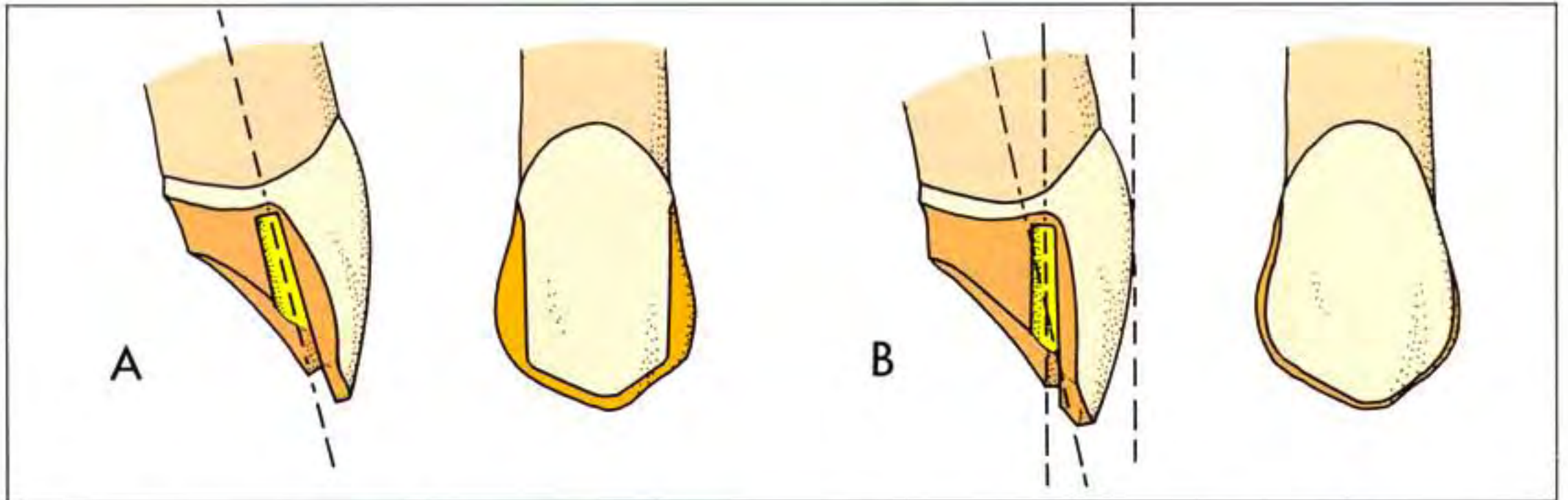
Fig. 1-26 Making the path of insertion of an anterior three-quarter crown parallel with the long axis of the tooth would result in an unnecessary display of metal (A). The preferred path of insertion for an anterior preparation parallels the incisal two-thirds of the labial surface (B). This not only will minimize the display of metal, but allow the grooves to be longer and more retentive.
