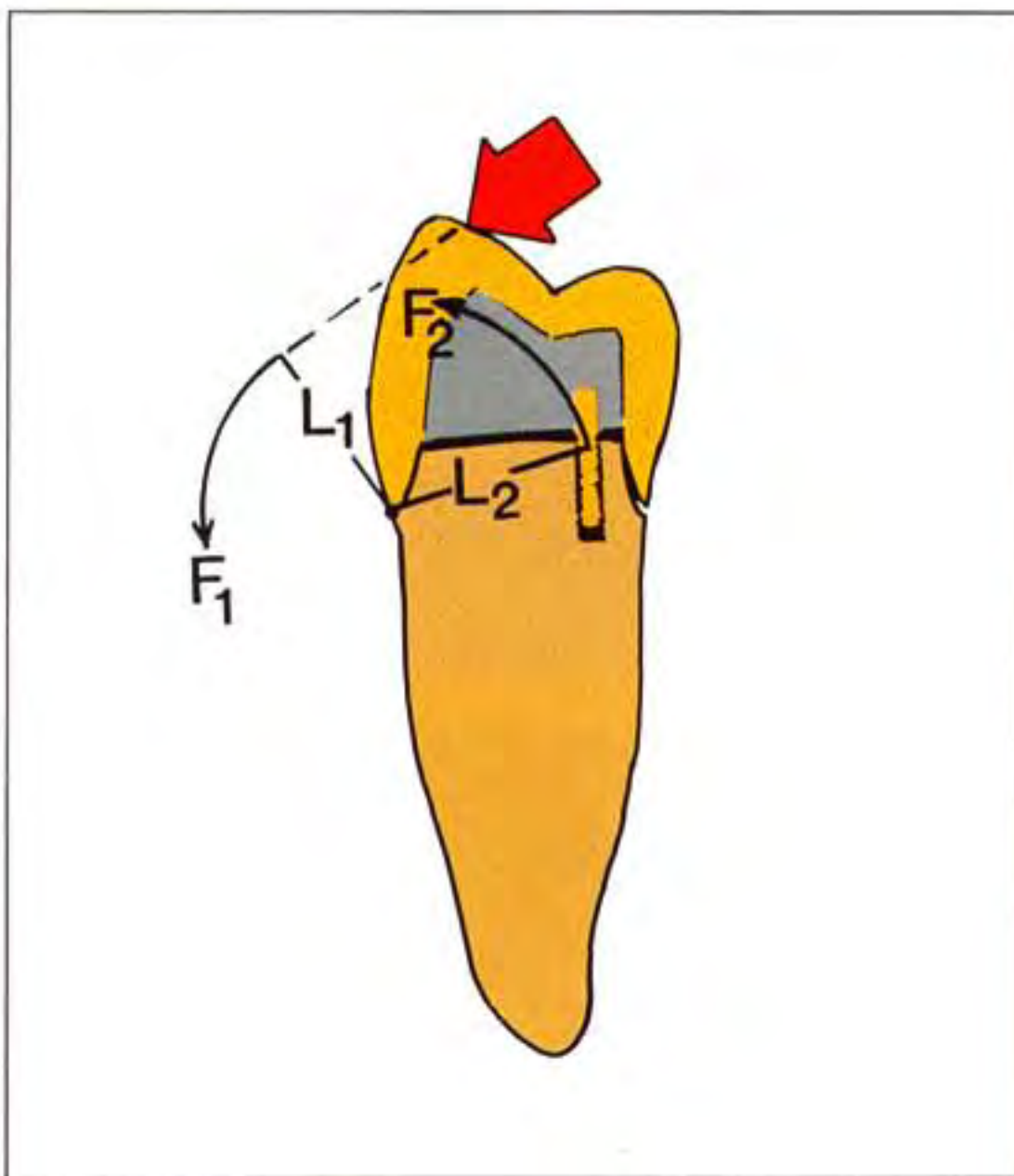
Fig. 16-36a A pin-retained amalgam core is inadequate for this narrow tooth. The dislodging force ( F_2 ) at the pinhole is about as great as the applied force ( F_1 ) because the lever arms ( L_1 and L_2 ) are nearly equal.
