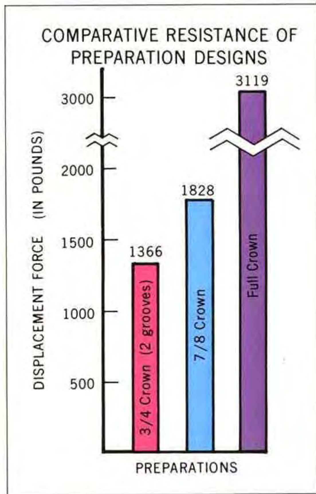
Fig. 9-2 Resistance values for the seven-eighths crown, the three-quarter crown, and the full veneer crown. 5
