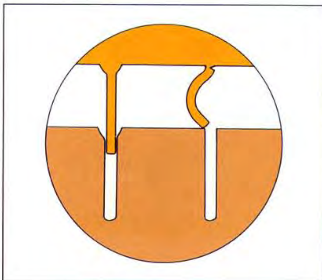
Fig. 16-15 The hole on the left has a small bevel at its mouth, which guides the pin to place. Without a beveled opening, the pin may fail to enter its hole, and be distorted ( right ).
