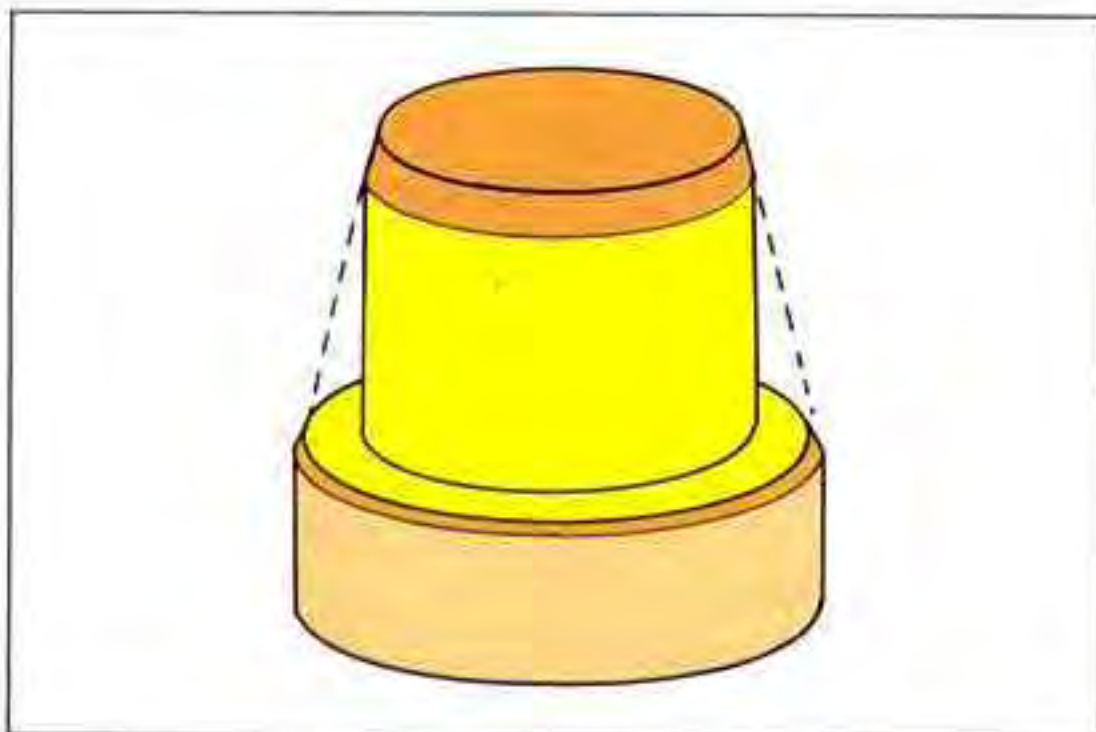
Fig. 16-11 An overtapered axial wall (broken outline) has been made more retentive by creating a gingival shoulder. This allows the vertical walls to be more nearly parallel.
