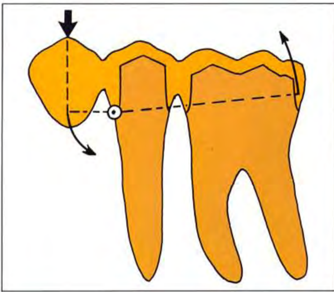
Fig. 17-4 An impact on a cantilevered pontic produces a strong lifting force on the distal retainer. Resistance can be increased by adding facial and lingual grooves, and by making the axial surface that is most distant from the pontic as nearly parallel with the wall nearest to the pontic as possible. The wall nearest the pontic must be as long as possible, thereby lowering the fulcrum and increasing the angle at which the arc of displacement strikes the distal wall.
