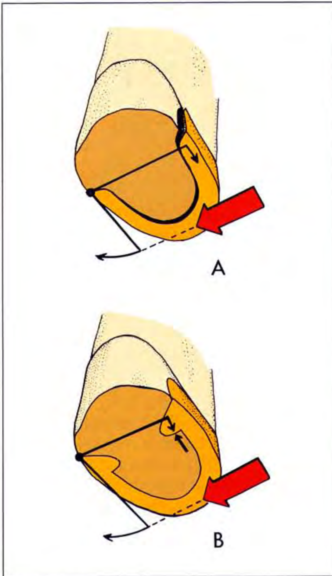
Fig. 1-23 A partial veneer crown which has no grooves (A) has little resistance to rotation around a vertical axis. When grooves are present, their lingual walls provide resistance by blocking the arc of rotation (B).
