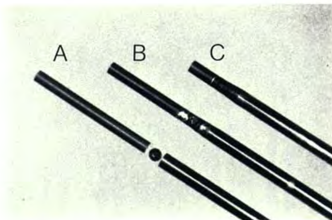
Fig. 3-4 A tungsten carbide dowel ( A, left ) is attached to a steel rod ( A, right ) with a small piece of solder interposed. The soldered carbide tip is machined ( B ) and shortened ( C ) to form the blank from which the bur will be cut.*
