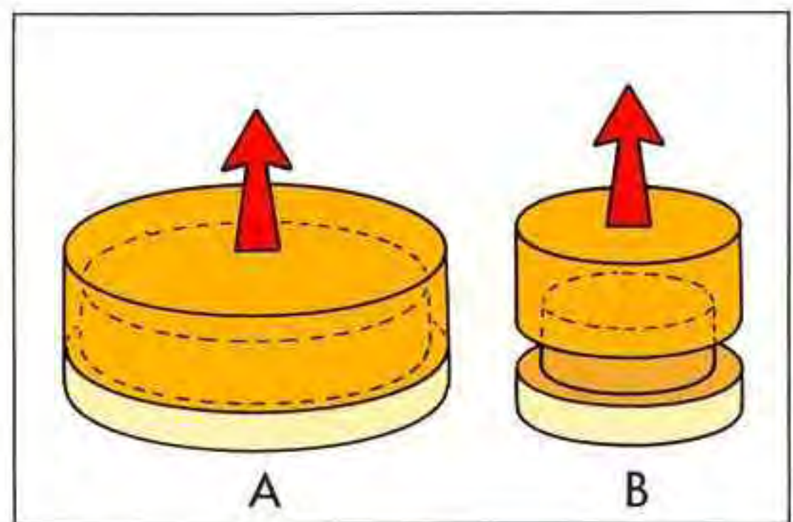
Fig. 1-11 Of two preparations of equal height and taper, the wider (A) will have greater retention than the narrower (B). Doubling the diameter of a preparation doubles the area of its axial walls under shear, and quadruples the area of the occlusal surface, where the cement is under tension.
